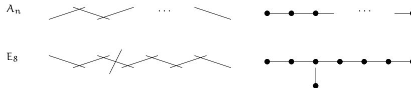
FIGURE 22.2. The exceptional divisors for resolutions of some ADE surface singularities, and their corresponding dual graphs (see Remark 22.4.3)
